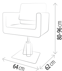
SQUARE Cadeira Cabeleireiro REF. MA6926-A85 (32 kg)
